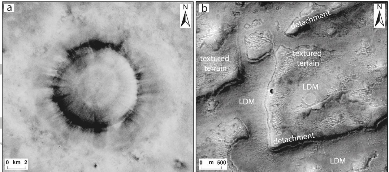
Figure 4: Latitude Dependent Mantle (LDM) vs. textured terrain. (a) Smoothened, subdued topography by LDM from 40°–44°N to 78°N. (P17_007612_2447_XN_64N024W). (b) Patches of textured terrain on Acidalia Colles region between 36° – 43°N and 79°N. Detachment of mantle material and/or Viscous Flow Features (VFF) is common at the inflexion point of the slope (B19_016895_2251_XN_45N024W).
