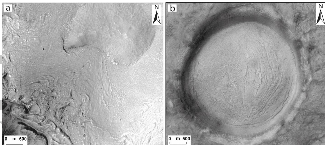
Figure 10: Large-scale Viscous Flow Features (VFF) between 36°N–53°N. (a) VFF inside a crater. (b) Crater with CCF, covered by LDM and textured terrain (B17_016407_2186_XI_38N021W).
