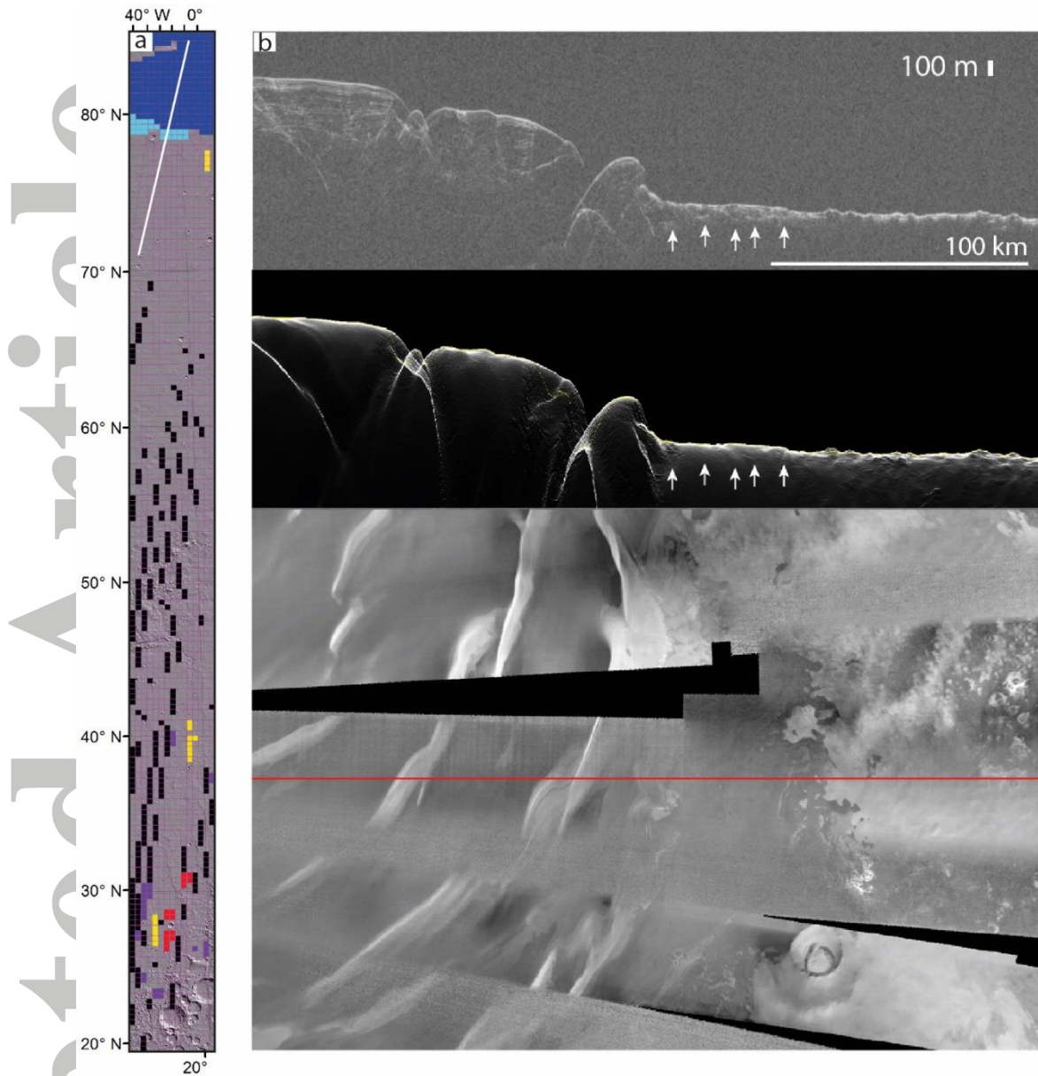
Figure 15: SHallow RADar observations along the Acidalia Planitia swath. a , SHARAD subsurface detections with MOLA hillshade background from latitude 20° to 84°N. Dark blue – NPLD, Light blue – near the NPLD, Red – high confidence detections, Purple – low confidence detections, Yellow – not correlated to subsurface detection, Black – no data. The white line shows the location of the radargram. b , Subsurface detection of ice near the NPLD (white arrows) (3703-02). The upper image is the radargram, the simulation is in the middle, the bottom image is MOLA DEM.
